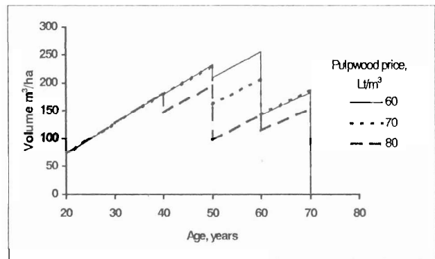
Figure 5. The impact of pulpwood price on optimal silvicultural regimes, using SEV(3%) criterion (H100 = 24, stocking level 20 = 0.9).
