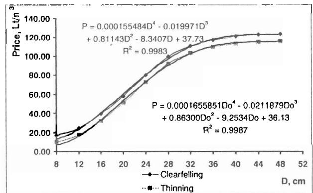
Figure 1. Prices curves for pine
